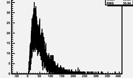
PT for positrons PT>25GeV and MET>40GeV
