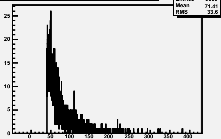
MET for electrons PT>25GeV and MET>40GeV
