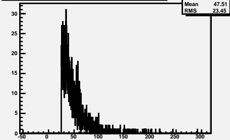
PT for positrons PT>25GeV and MET>40GeV
