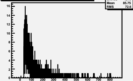
E for positrons PT>25GeV and MET>40GeV
