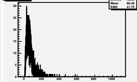
Electron Pt
