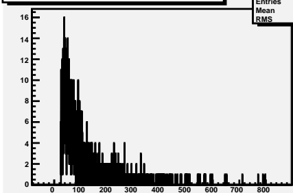
E for positrons PT>25GeV and MET>40GeV
