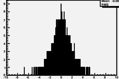
ElectronNeutrino_Eta
