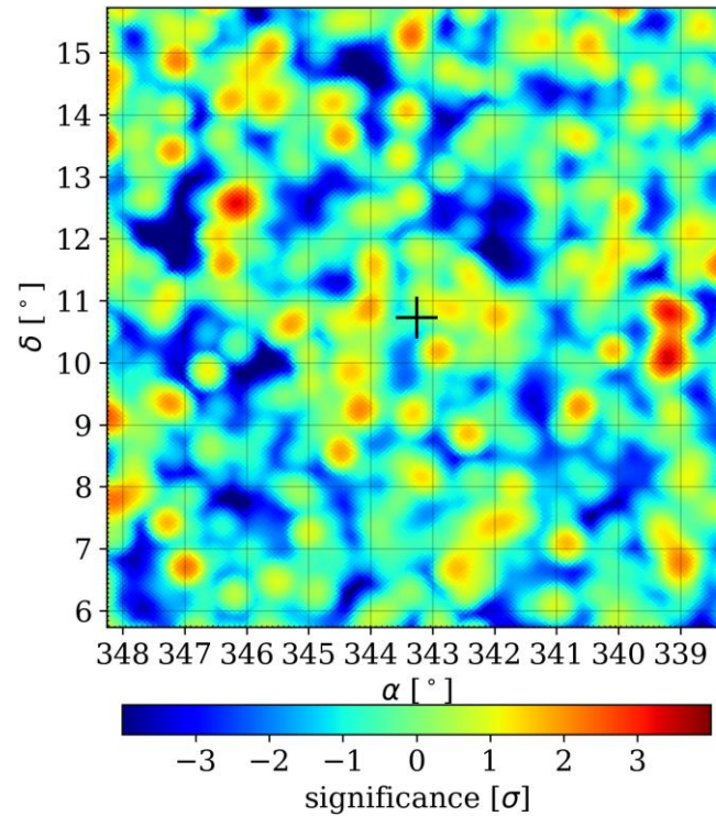
Transit on 6/19/19 (alert)
