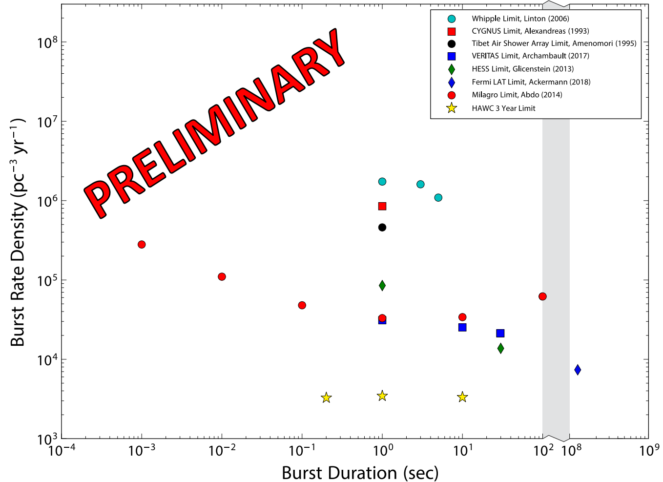
PBH Burst Rate Density Upper Limits
