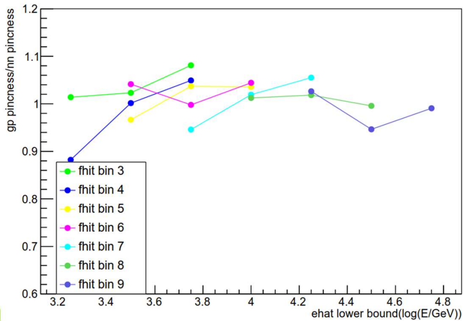
ratio of pincness
