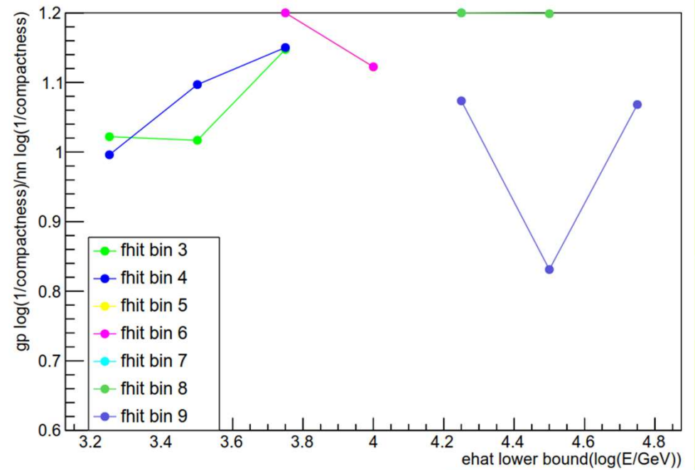
ratio of \log(1/\text{compactness})
