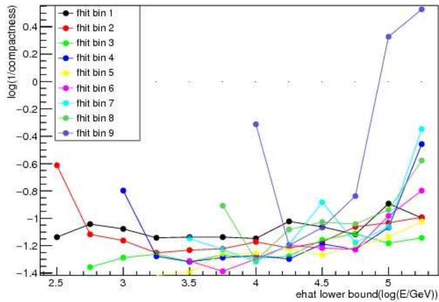
John log(1/compactness)
