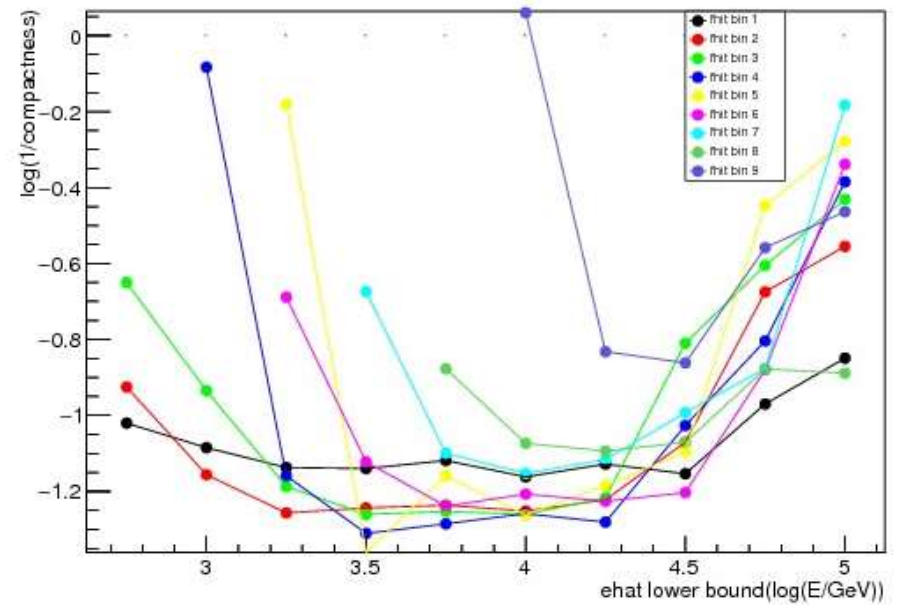
log(1/compactness)
