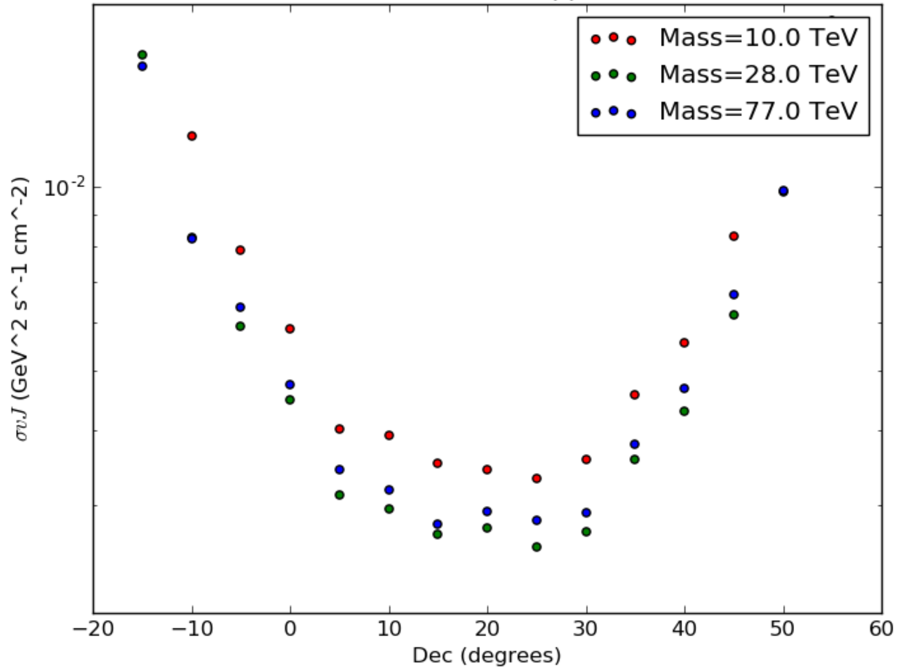
B Bbar Annihilation Upper Limits
